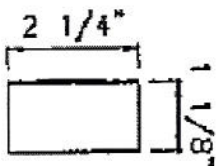
NO. 5 LATCHBOLT CUTOUT
