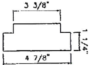
NO. 2 ASA STRIKE CUTOUT
